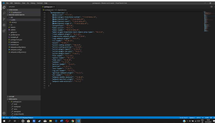
Рис. 3.6 – devDependencies
